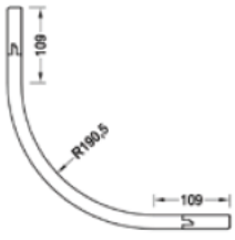
Curved Door 715 x 295 x 295mm
